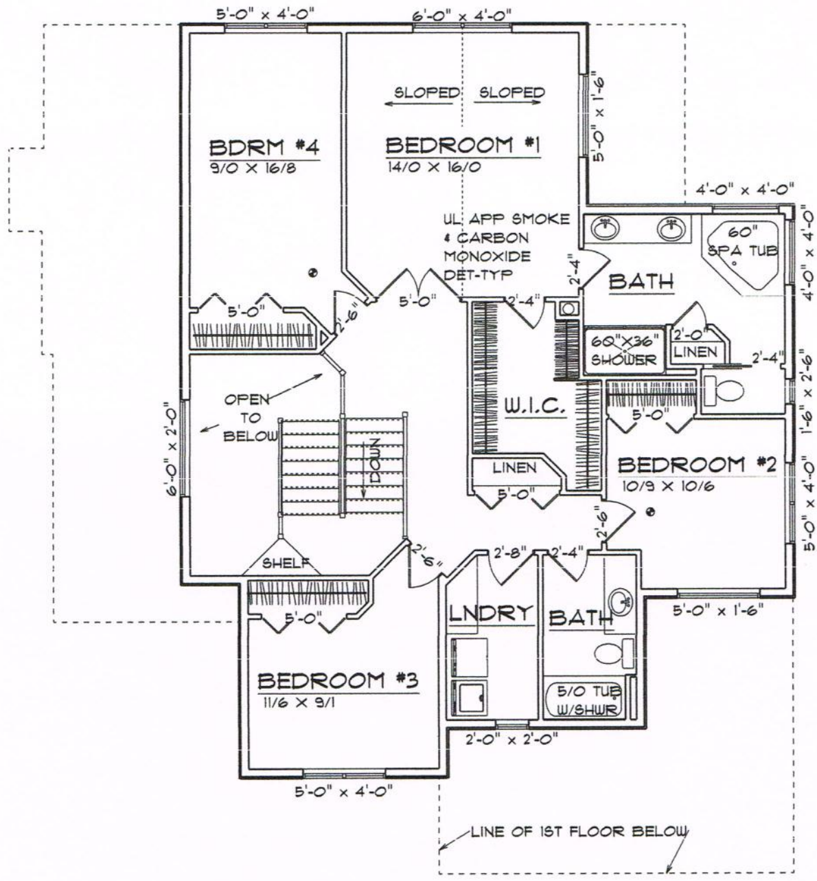
2ND FLOOR LAYOUT SCALE: 1/8" = 1'-0"
