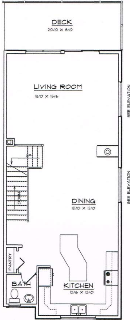
2ND FLOOR LAYOUT
