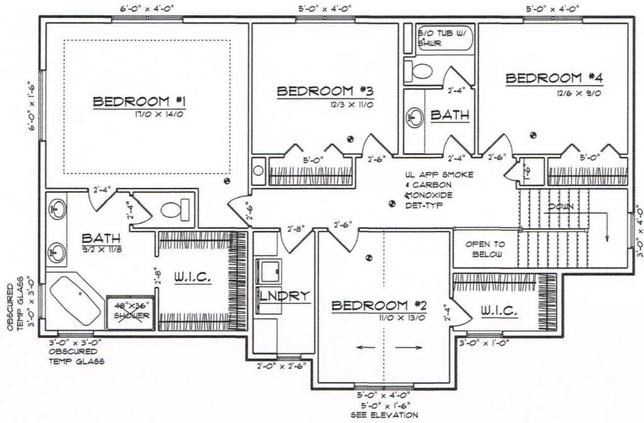
2ND FLOOR LAYOUT SCALE: 1/8" = 1'-0"
