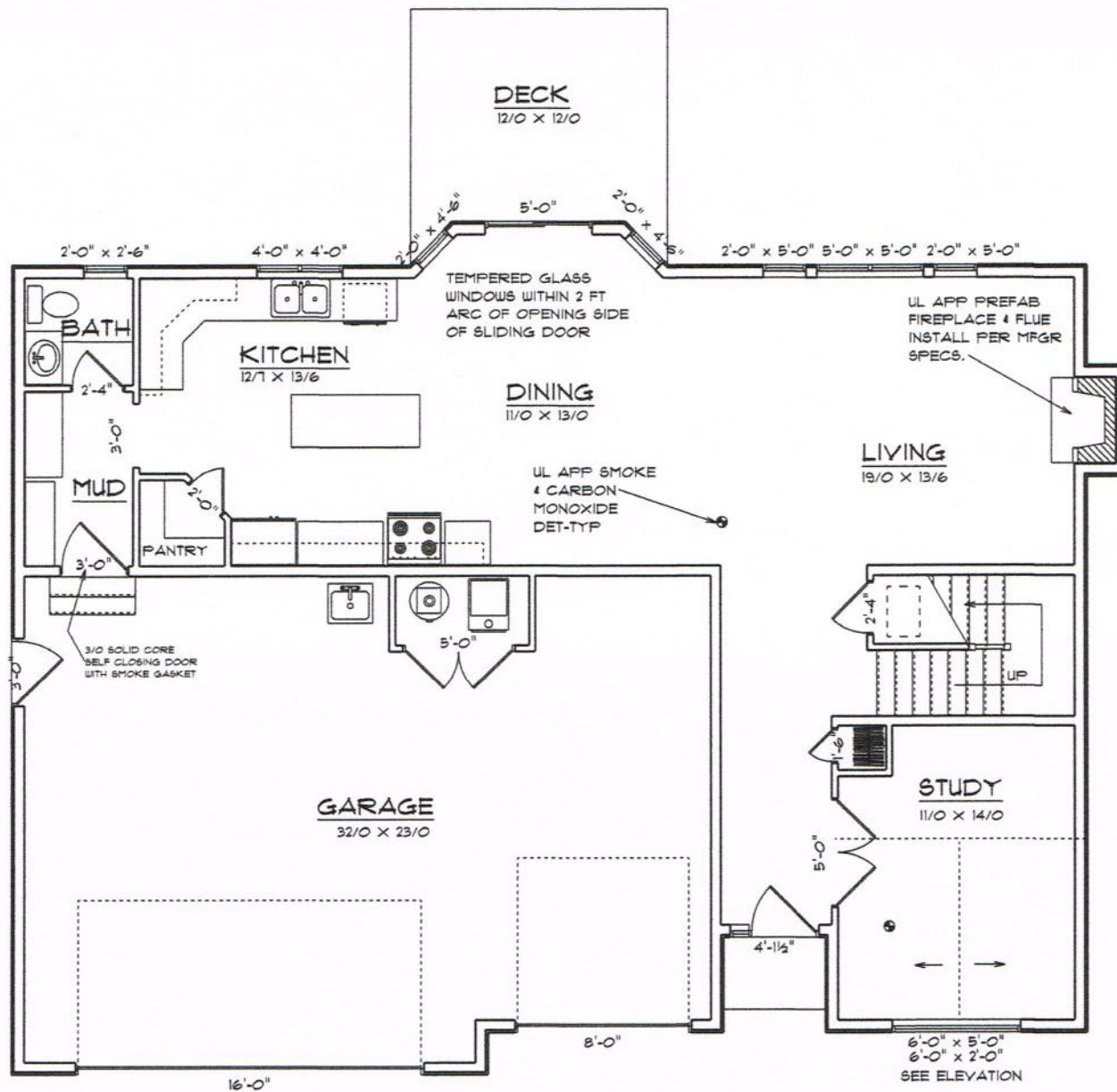
1ST FLOOR LAYOUT SCALE: 1/8" = 1'-0"
